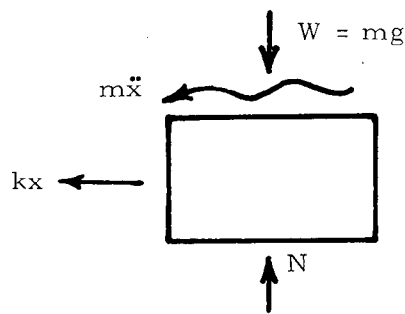
(a) Undamped single-degree-of-freedom system.
